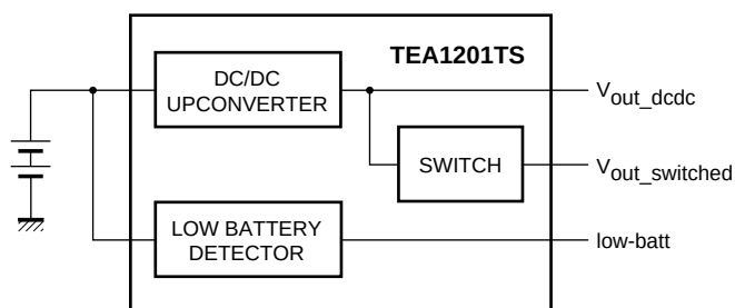
Equivalent block diagram
