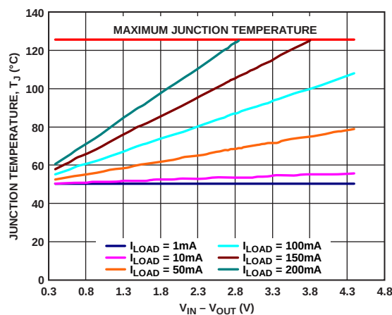
Figure 48. TSOT 500 mm 2 of PCB Copper, T_A = 50^\circ\text{C}
