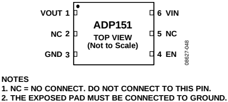
Figure 6. 6-Lead LFCSP Pin Configuration
