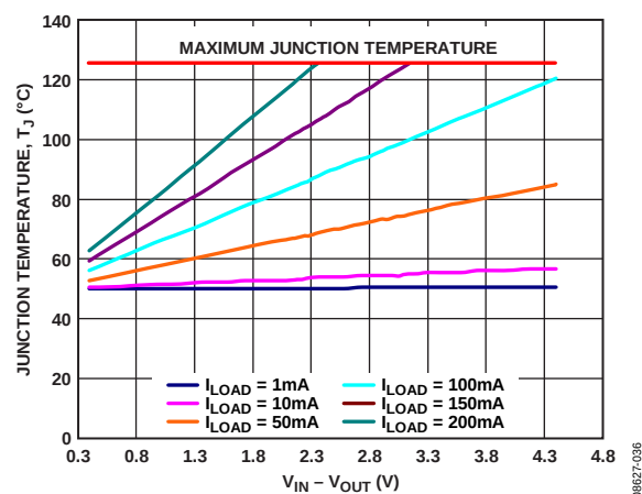
Figure 44. WLCSP 50 mm² of PCB Copper, T_A = 50^\circ\text{C}
