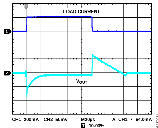
Figure 24. Load Transient Response, C_{IN} , C_{OUT} = 1\text{ μF} , I_{LOAD} = 1\text{ mA} to 200\text{ mA}
