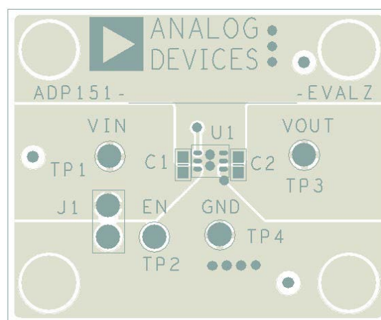
Figure 62. Example LFCSP PCB Layout
