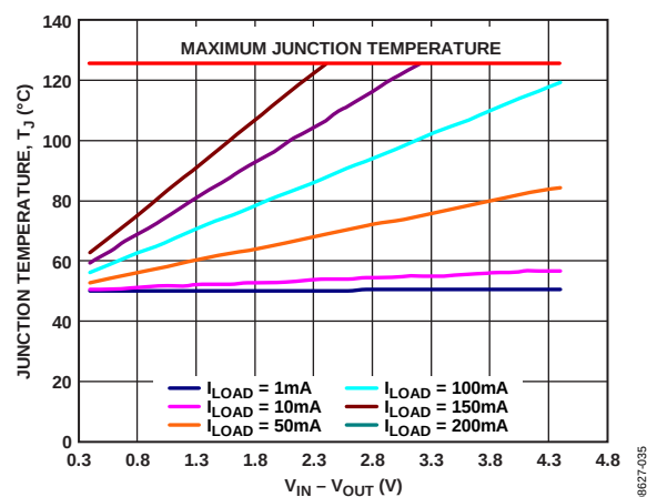
Figure 43. WLCSP 100 mm² of PCB Copper, T_A = 50^\circ\text{C}
