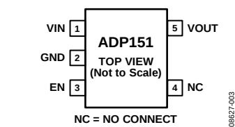
Figure 4. 5-Lead TSOT Pin Configuration
