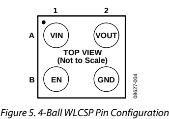
Figure 5. 4-Ball WLCSP Pin Configuration
