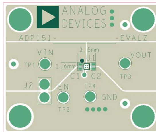
Figure 61. Example WLCSP PCB Layout
