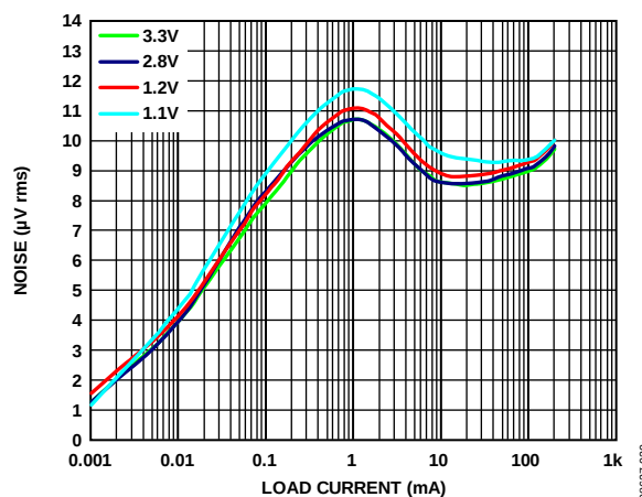
Figure 22. Output Noise vs. Load Current and Output Voltage, V_{IN} = 5\text{ V} , C_{OUT} = 1\text{ μF}
