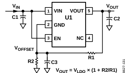
Figure 33. Adjustable LDO Using the ADP151
