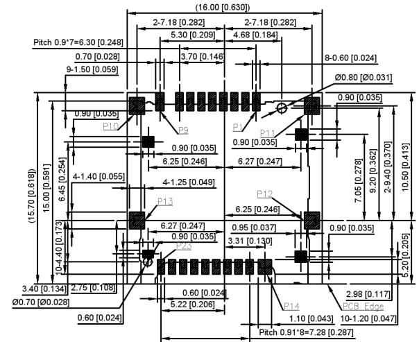
Recommended PCB Layout Top View (Tolerance \pm 0.05 )
