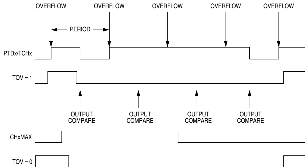
Figure 17-8. CHxMAX Latency
