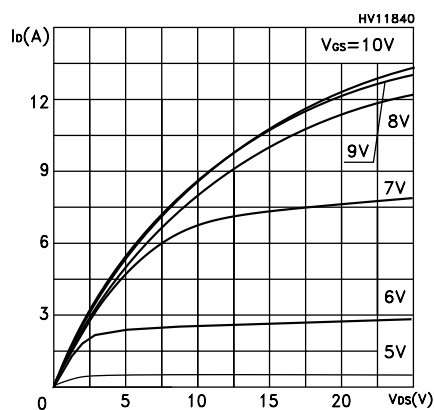
Figure 5. Output characteristics
