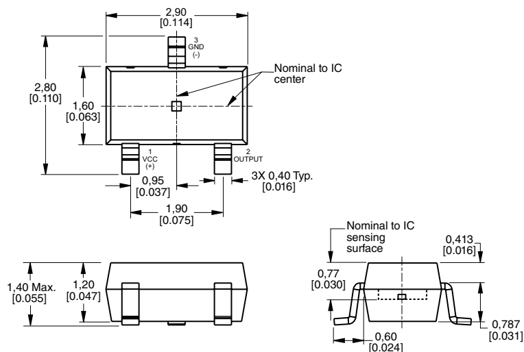
Sensor Showing Polarity
