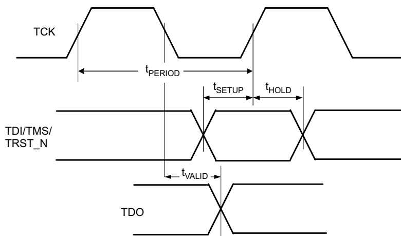
Figure 9-5. JTAG Timing
