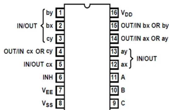
DIP16/SOP16/TSSOP16
