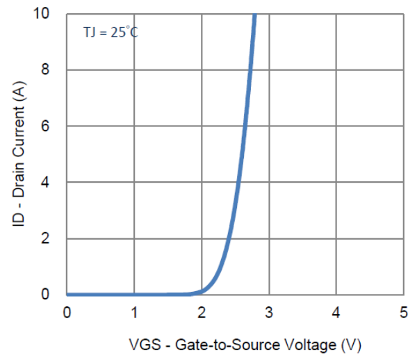
2. Transfer Characteristics
