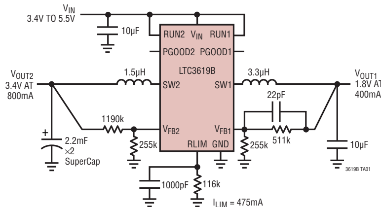
Dual Monolithic Buck Regulator in 10-Lead 3mm \times 3mm DFN
