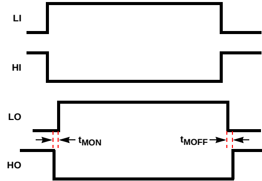
FIGURE 4. DELAY MATCHING
