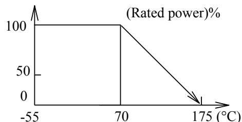
High Precision Resistor Coating Type (RE) Power - Temperature Curve
