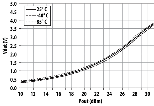
Figure 17. Over-temperature Vdet vs Output Power at 756 MHz
