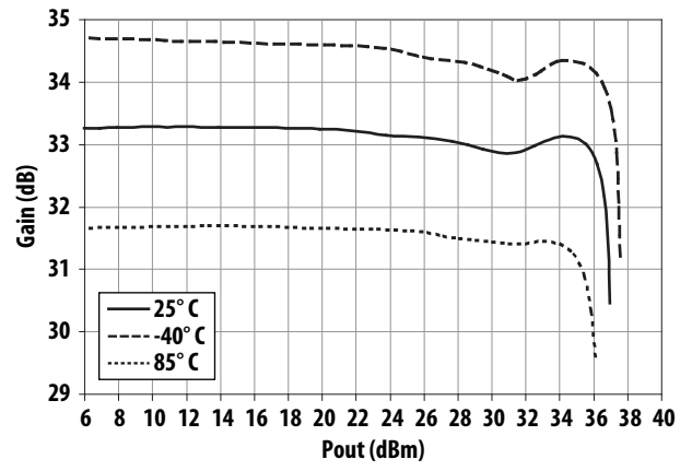
Figure 18. Over-temperature CW Gain vs Output Power at 756 MHz
