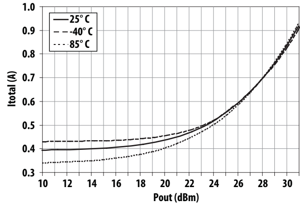
Figure 8. Over-temperature I_{dd\_total} vs Output Power at 728 MHz
