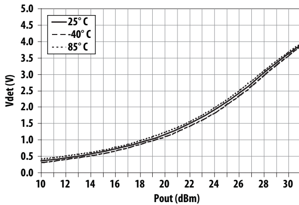
Figure 9. Over-temperature V_{det} vs Output Power at 728 MHz
