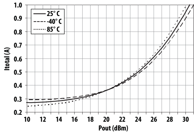
Figure 32. Over-temperature Idd_total vs Output Power at 706 MHz
