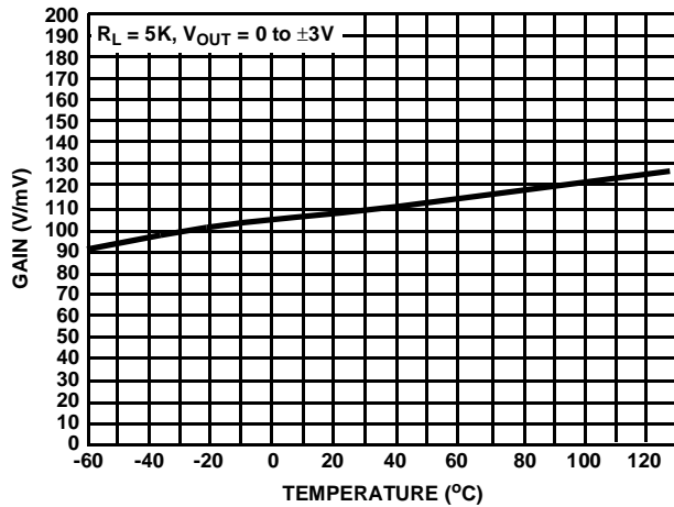
FIGURE 13. OPEN LOOP GAIN vs TEMPERATURE R_L = 5K , V_{OUT} = 0 to \pm 3V
