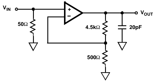
FIGURE 1. LARGE AND SMALL SIGNAL RESPONSE TEST CIRCUIT
