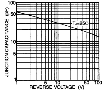
FIG.4-TYPICAL JUNCTION CAPACITANCE
