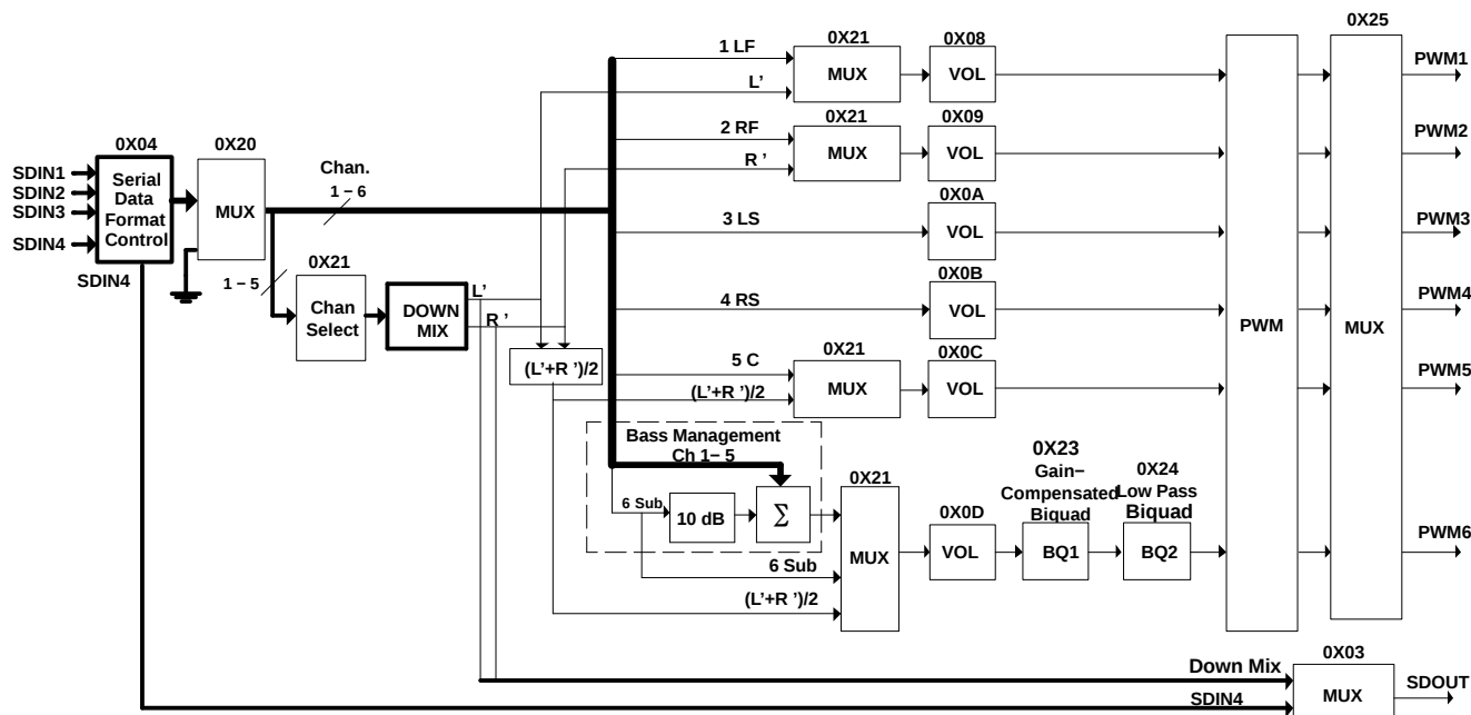
Figure 2. TAS5086 Data Flow Diagram With I 2 C Registers
