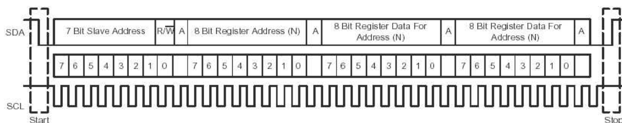
Figure 10. Typical I 2 C Sequence
