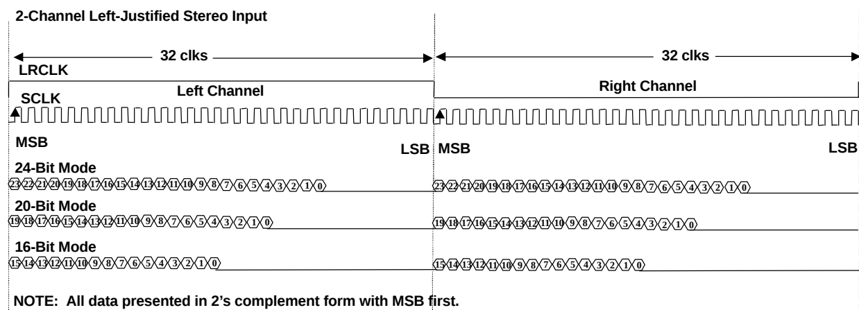
Figure 6. Left Justified 64 Fs Format
