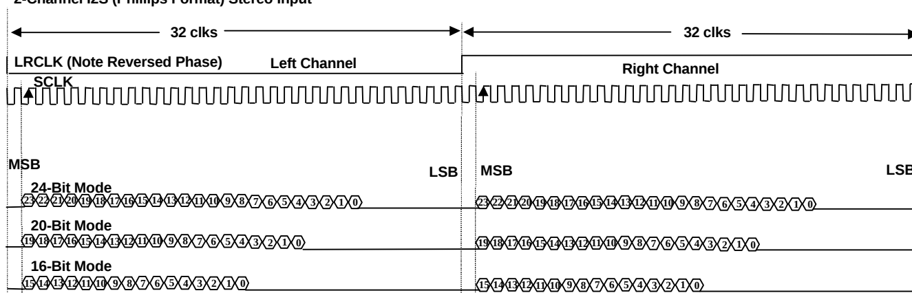
2-Channel I2S (Phillips Format) Stereo Input
