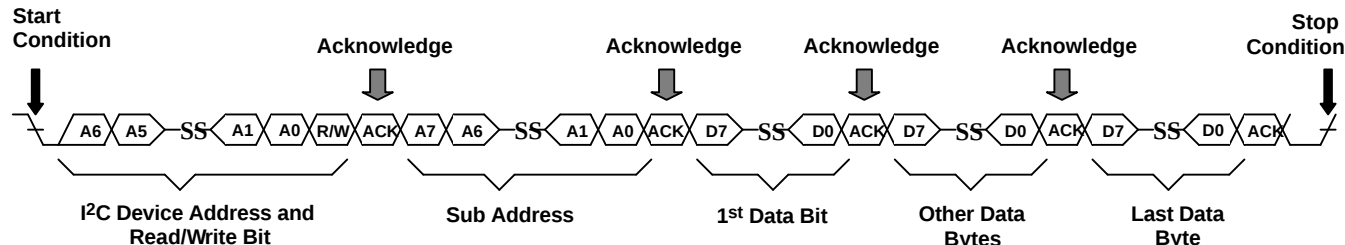
Figure 12. Multiple Byte Write Transfer
