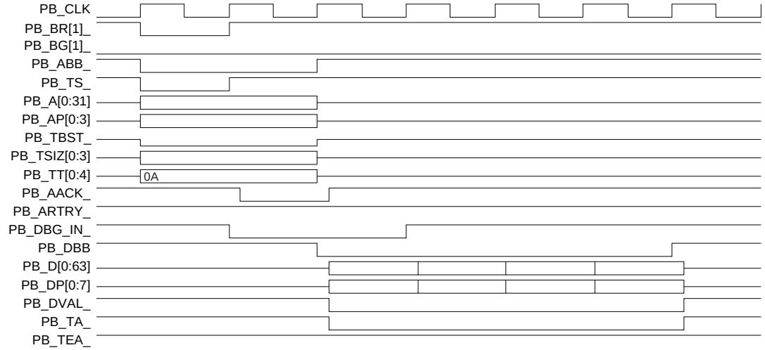
Figure 13: PB Master Interface Burst Read
