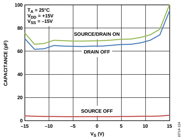
Figure 30. ADG5206 Capacitance vs. Source Voltage, ±15 V Dual Supply
