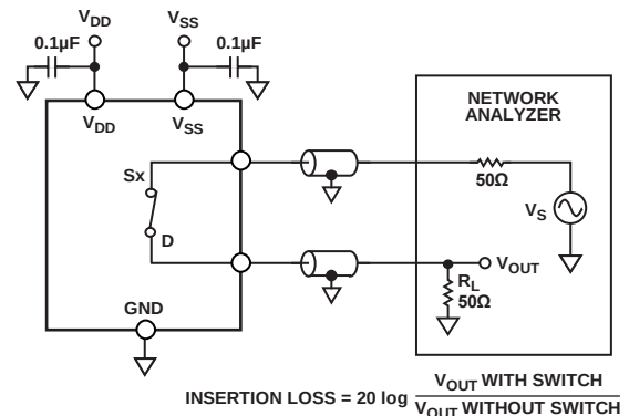
Figure 41. Bandwidth
