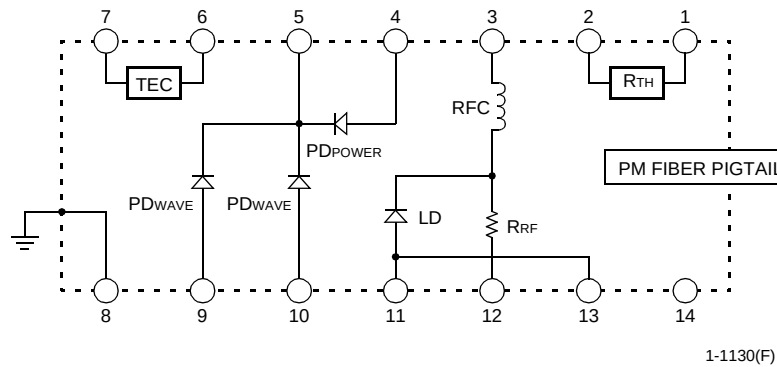
Figure 3. D2587P Circuit Schematic
