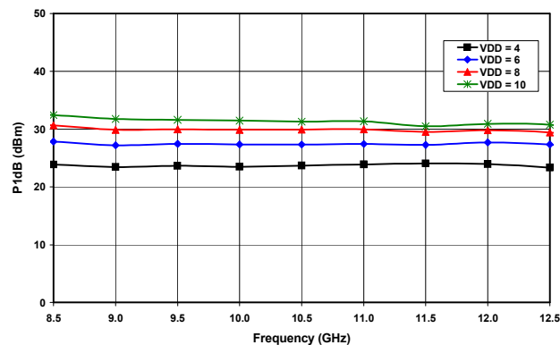
Figure 2. 1dB Compression Point vs. Drain Voltage
