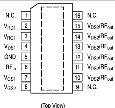
Figure 2. Pin Connections
