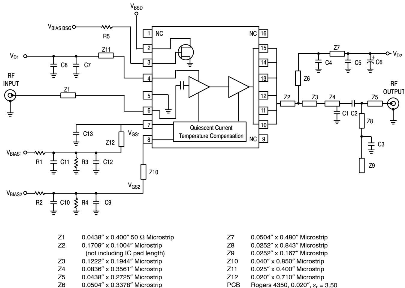
Figure 3. MHVIC915NR2 Test Circuit Schematic
