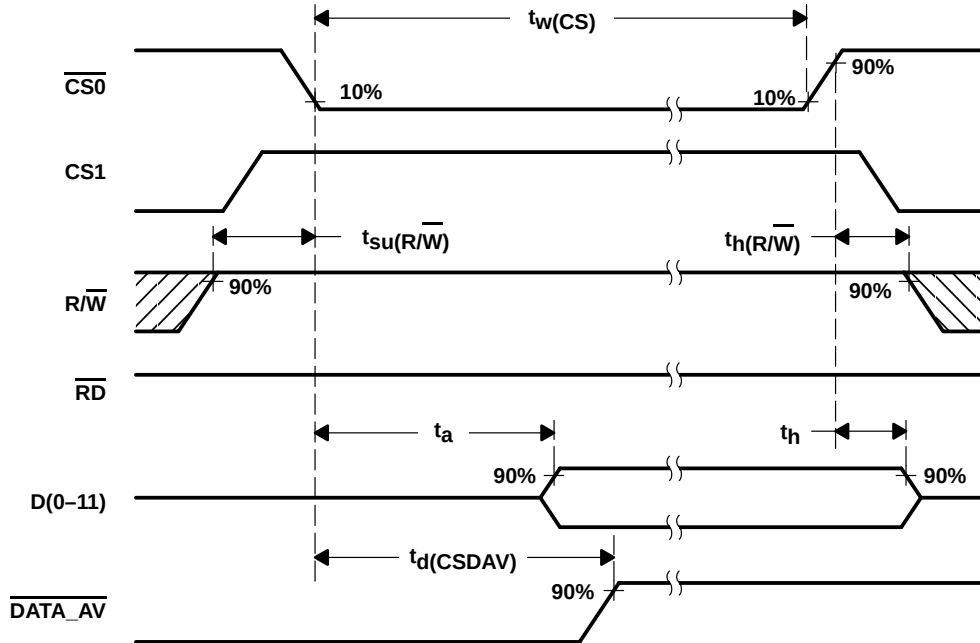
Figure 36. Read Timing Diagram Using \overline{RD} ( \overline{CS0} -controlled)
