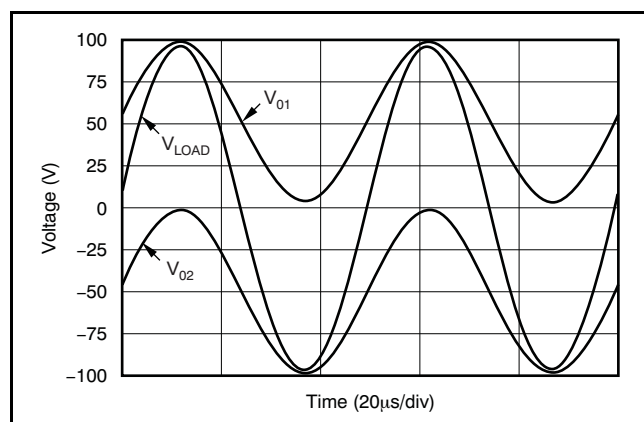
Figure 77. 195V pp On 3.75k \Omega Load to Ground 20kHz, Uses 3 OPA454s, 100V Supplies
