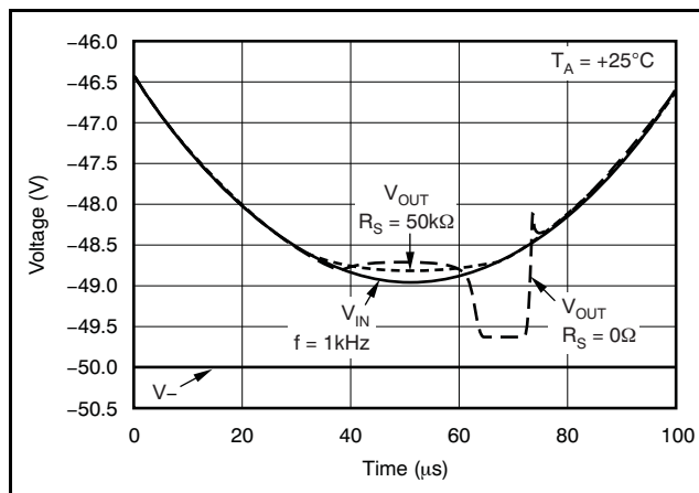
Figure 63. Output Voltage With Input Voltage Down To (V_-) + 1\text{ V}
