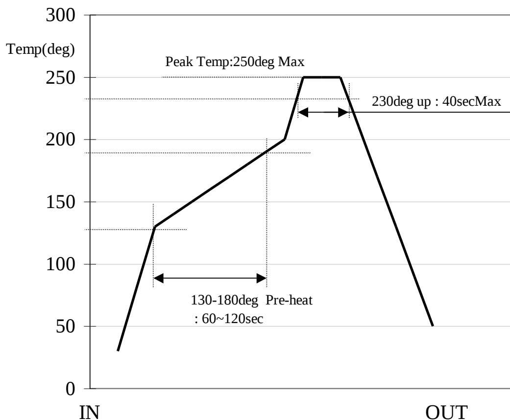
Recommended Reflow Profile
