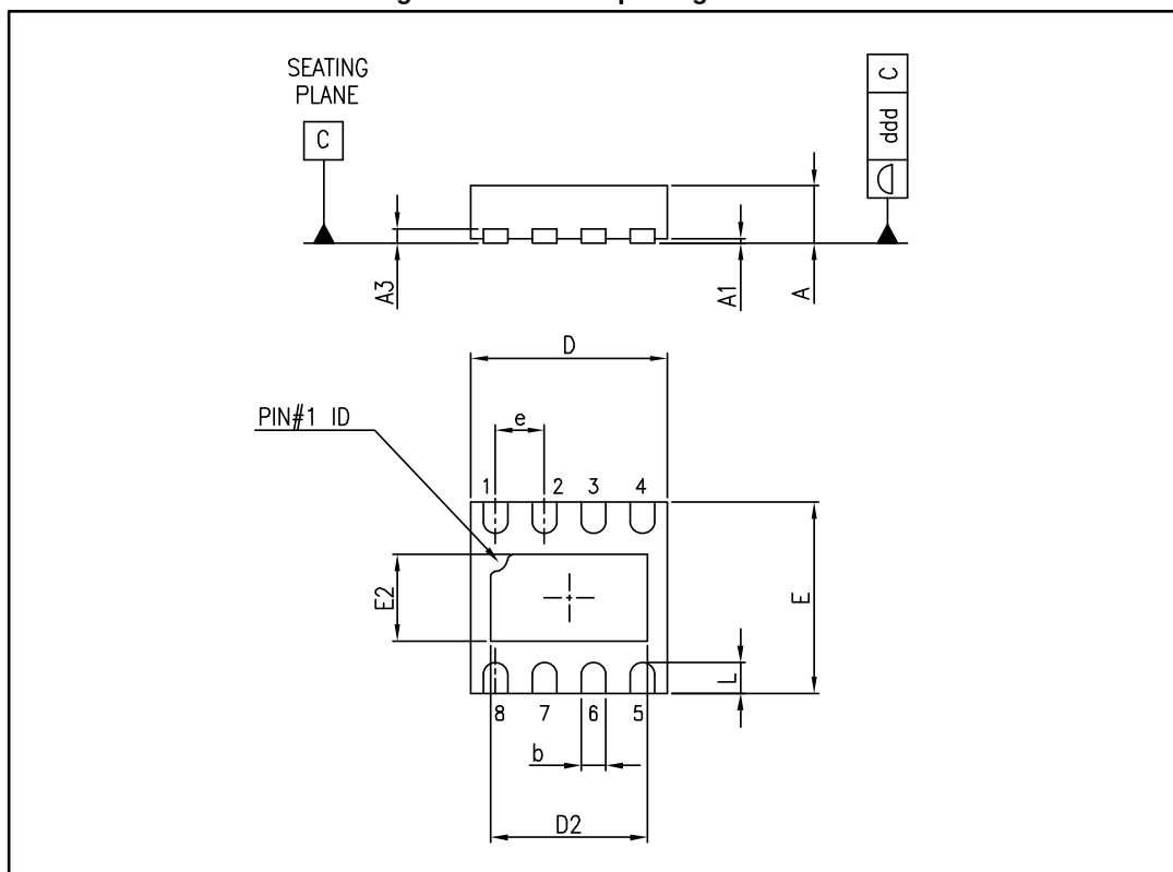
Figure 9: DFN8 2x2 package outline
