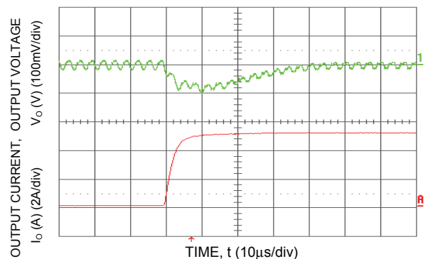
Figure 12. Transient Response to Dynamic Load Change from 50% to 100% of full load ( V_o = 3.3 Vdc , C_{ext} = 2x150 \mu F Polymer Capacitors).
