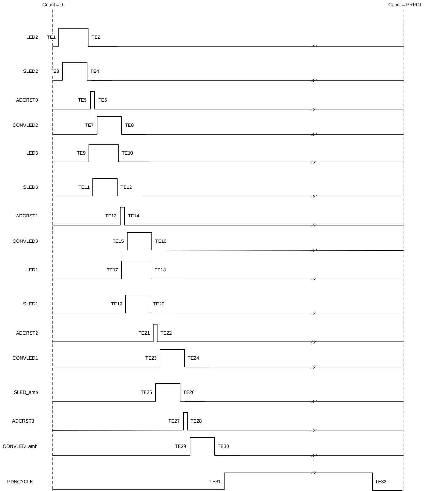
Figure 32. Timing Diagram
