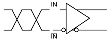
Figure 16. Differential Inputs Driven Differentially
