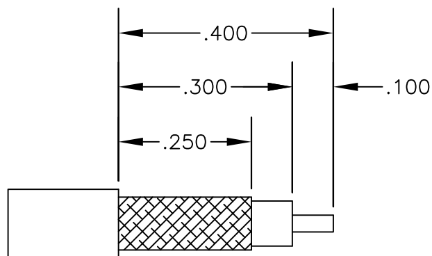
STRIPPING DIMENSIONS
