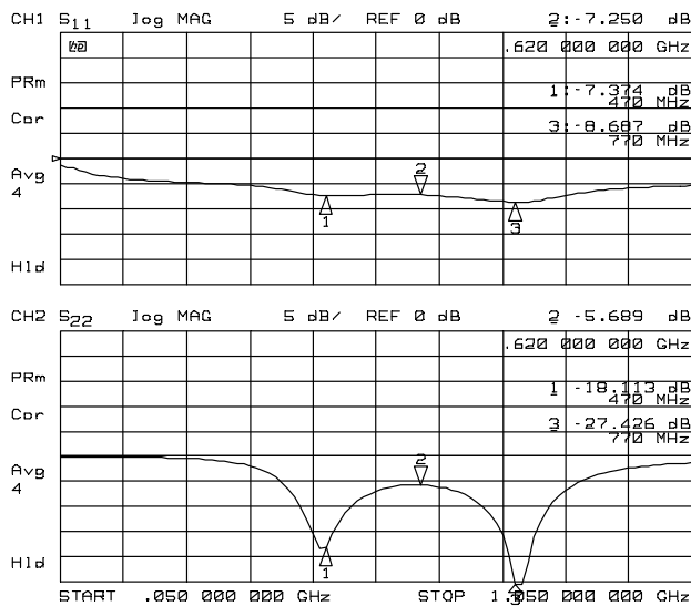
S 11 , S 22
