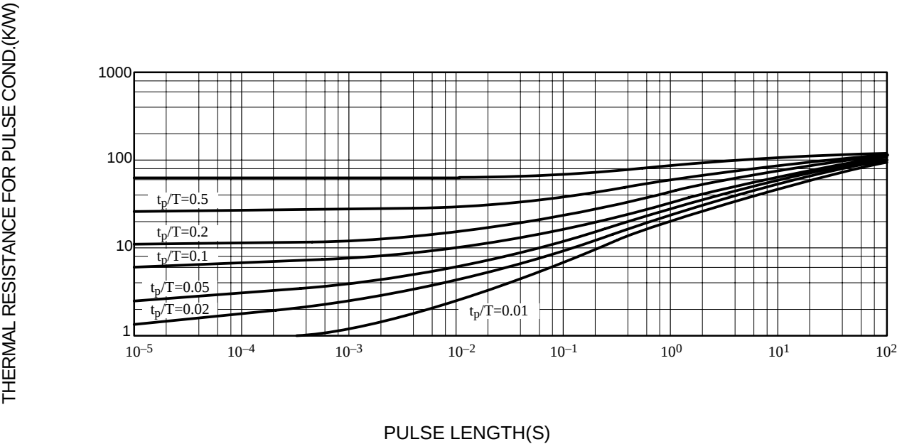
FIG.3 – THERMAL RESPONSE
