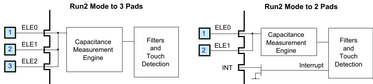
Figure 15. Electrode/Pad Connections in Area Detection Mode
