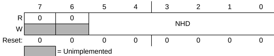
Figure 28. Noise Half Delta Register
