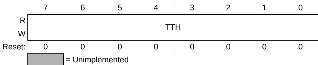
Figure 30. Touch Threshold Register
