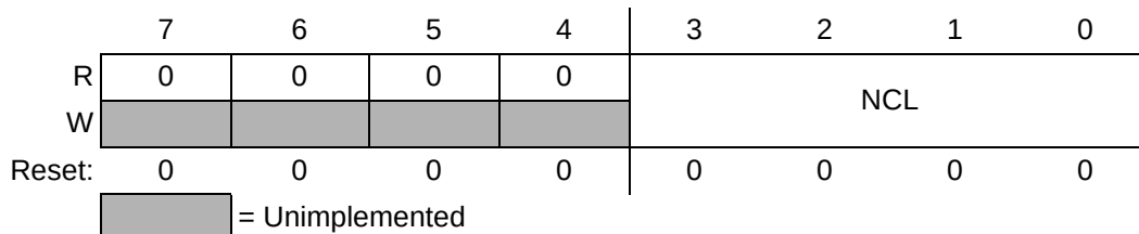
Figure 29. Noise Count Limit Register
