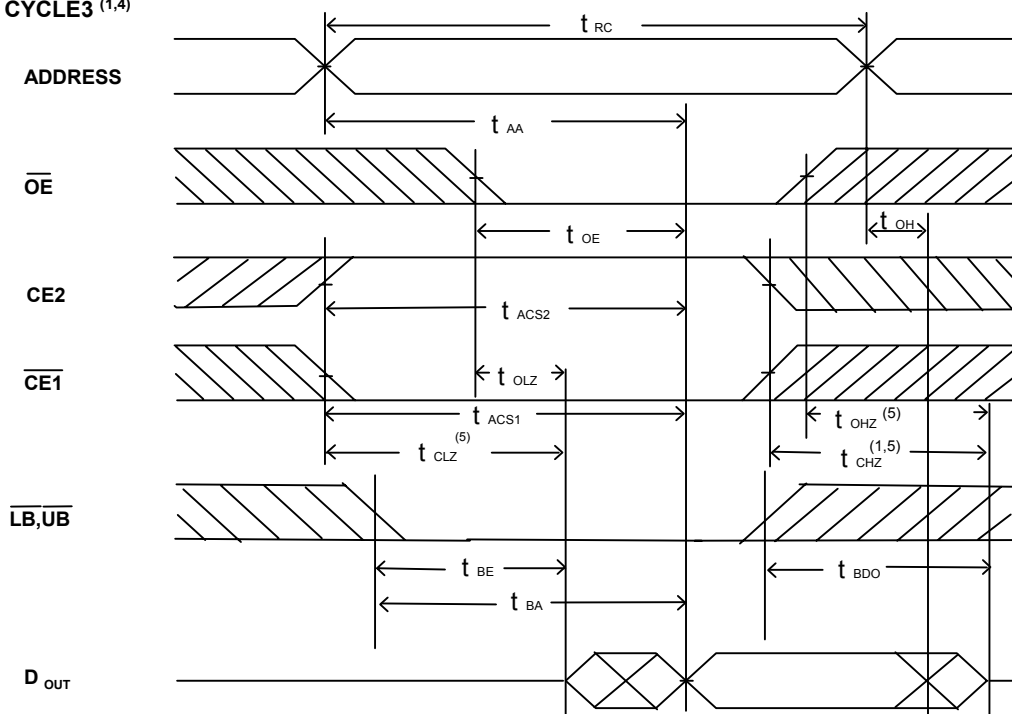
READ CYCLE3 (1,4)
