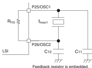
Figure:1.5.2 External Oscillator 1
