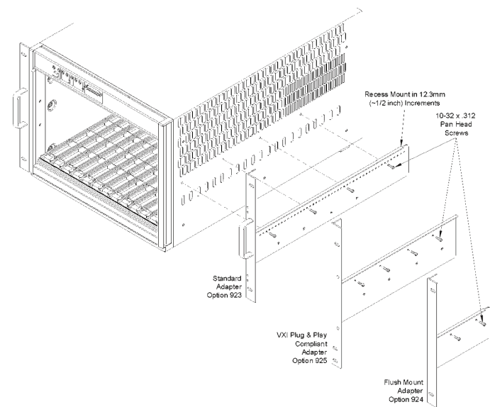
Attaching the Rack Mount Adapter to the Mainframe
