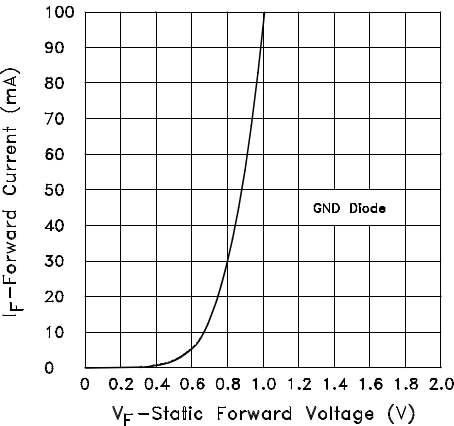
I_F vs V_F Characteristic
