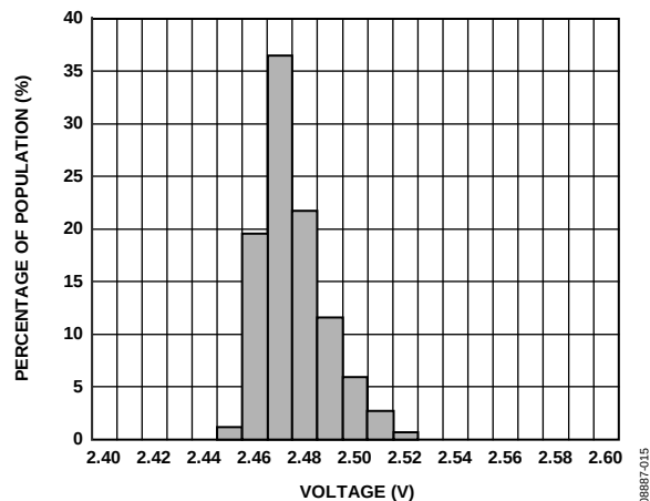
Figure 13. V_{TEMP} Output at 25°C ( V_{RATIO} = 5\text{ V} )
