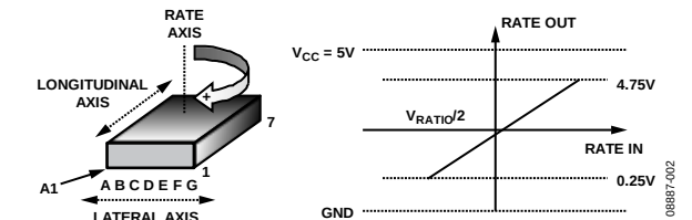
Figure 2. RATEOUT Signal Increases with Clockwise Rotation
