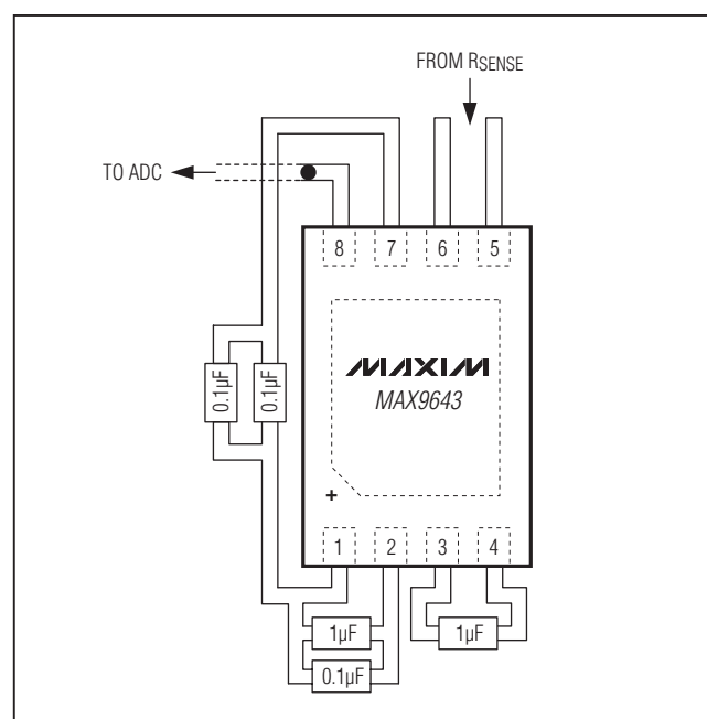
Figure 1. PCB Layout
