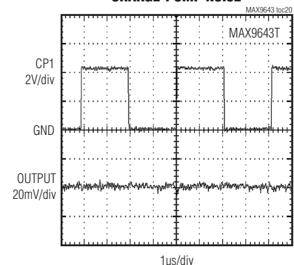
CHARGE-PUMP NOISE
