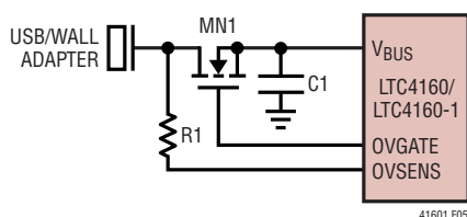
Figure 5. Overvoltage Protection
