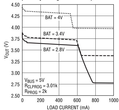
V_{OUT} Voltage vs Load Current (Battery Charger Disabled)
