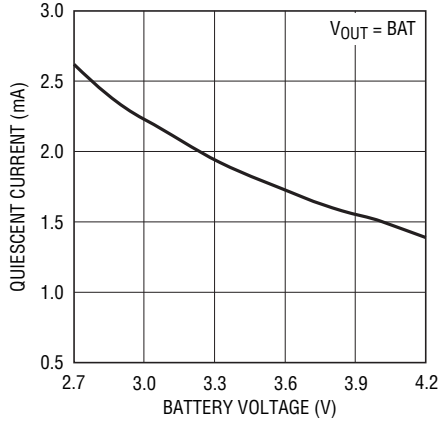
OTG Boost Quiescent Current vs Battery Voltage
