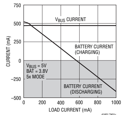
Battery and V_{BUS} Currents vs Load Current
