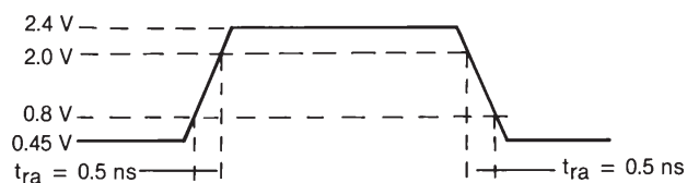
Figure 10 : Input pulse characteristics.
