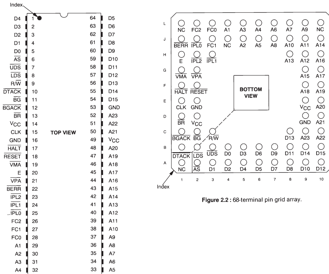
Figure 2.1 : 64-pin dual-in-line package.
