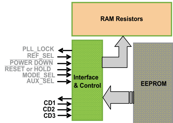
Figure 14. Using CD1, CD2 to Control What is Copied From EEPROM Into RAM Registers at Power Up
