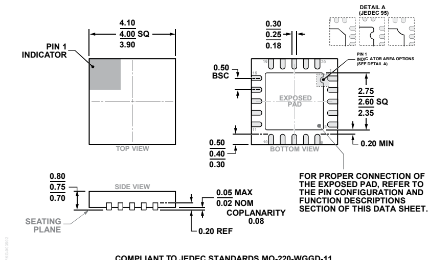
COMPLIANT TO JEDEC STANDARDS MO-220-WGGD-11. Figure 110. 20-Lead Lead Frame Chip Scale Package [LFCSP] 4 mm × 4 mm Body and 0.75 mm Package Height (CP-20-8) Dimensions shown in millimeters
