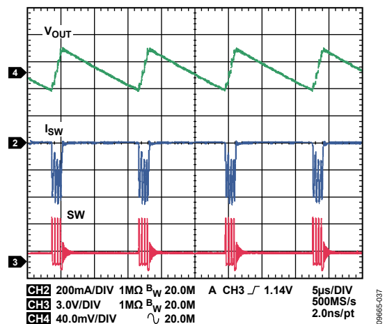
Figure 37. Typical Waveforms, V_{OUT1} = 1.2\text{ V} , I_{OUT1} = 30\text{ mA} , Auto Mode
