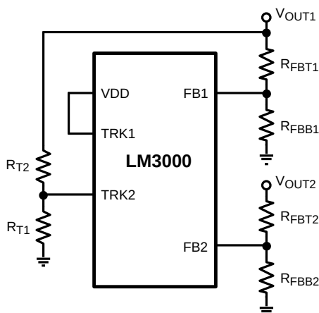
Figure 20. Tracking with V_{OUT1} Controlling V_{OUT2}
