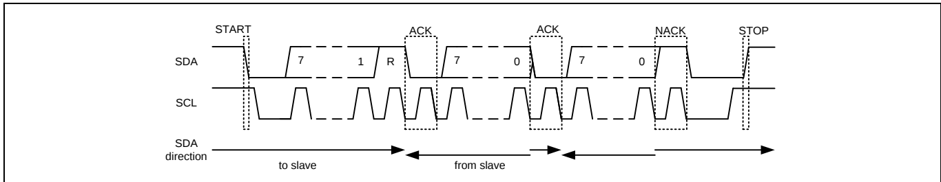
Figure 28. Read Transaction
