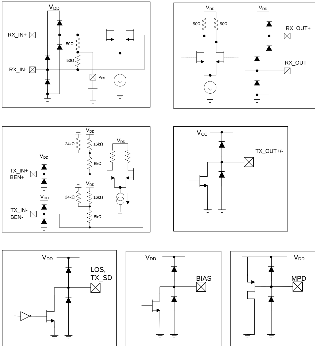
Figure 29. Interface Diagrams
