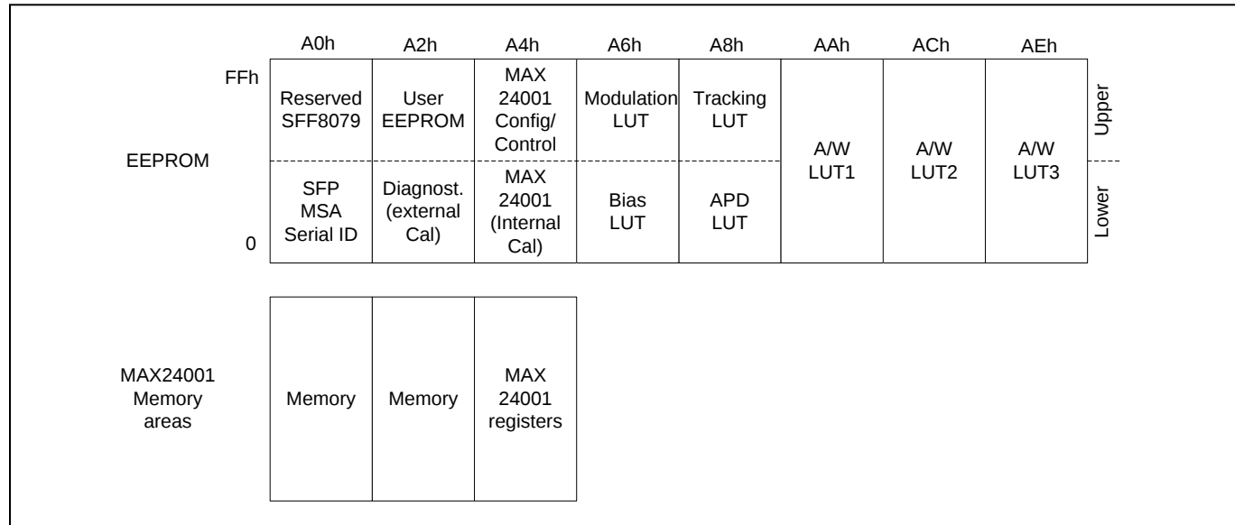
Figure 24. Address Map
