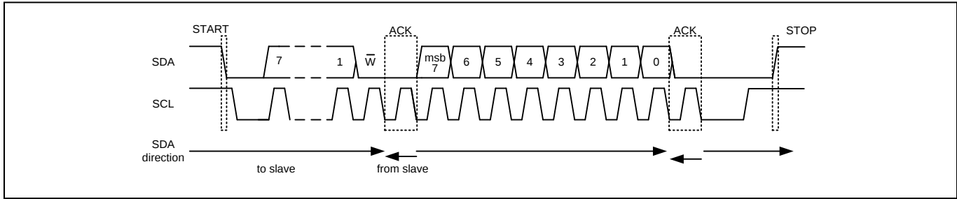
Figure 27. Write Transaction
