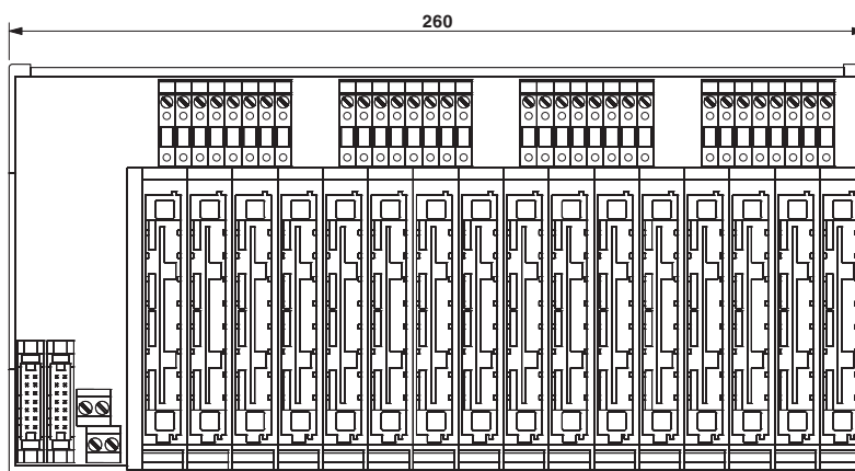
Dimensional drawing
