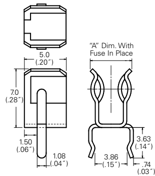
111 501 / 111 506 Device Dimensions
