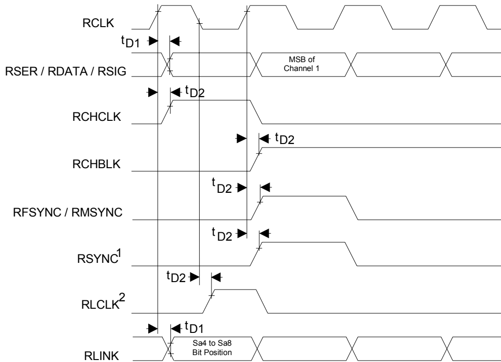
Figure 38-9. Receive Side Timing, Elastic Store Disabled (E1 Mode)
