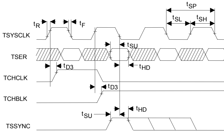
Figure 38-14. Transmit Side Timing, Elastic Store Enabled
