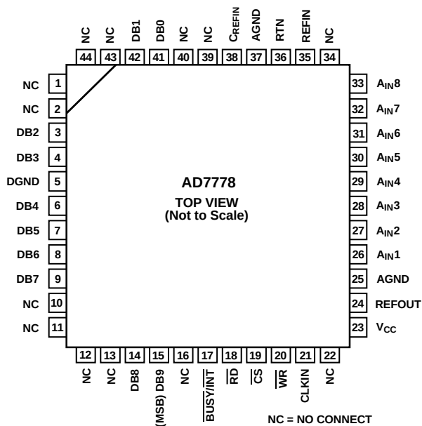
44-Pin PQFP
