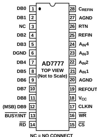
28-Pin DIP & SOIC
