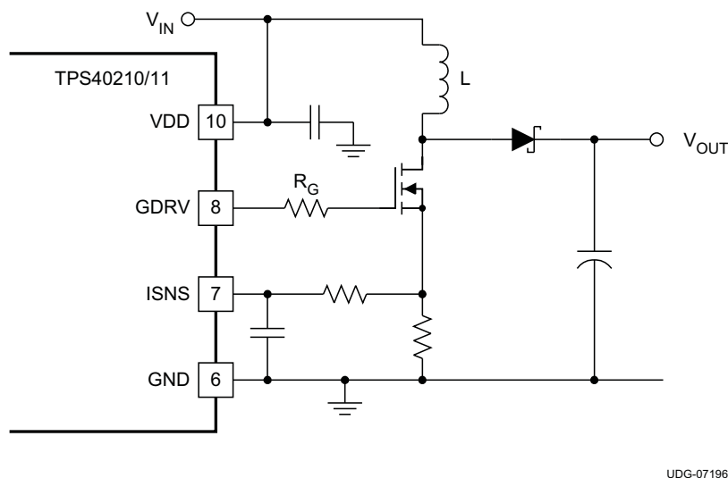
Figure 28. Gate Drive Resistor
