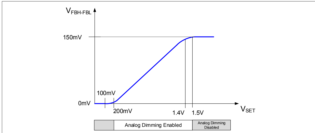
Figure 25 Analog Dimming Overview
